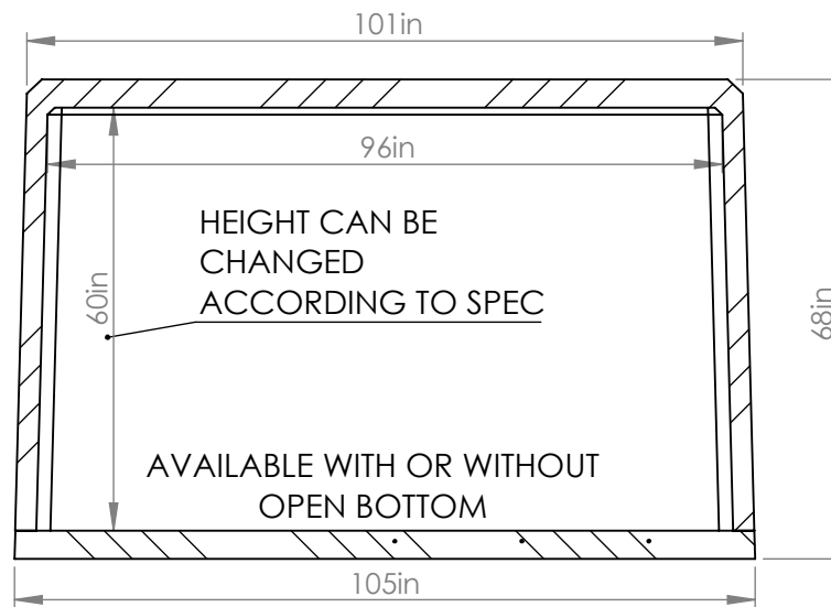
SECTION C-C
